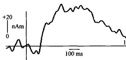
Fig. 3. Results of dipole source analysis of the HN minus MN difference waveform at the 450–650 ms time window. The left side shows the source activity waveforms and the right side shows the mean dipole location. This dipole is also approximately located in the right hippocampus ( x = 17.7 , y = -38.0 , z = 5.8 ).
